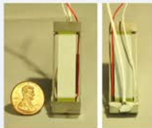
Picture of the strain gages attached preload piezo actuator
